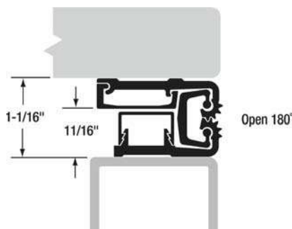
Closed Position
