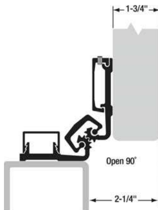
90° Open Position
