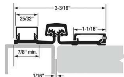
180° Open Position
