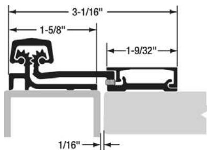
Closed Position
