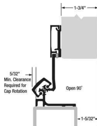
180° Open Position
