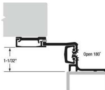
90° Open Position
