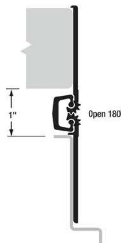
180° Open Position
